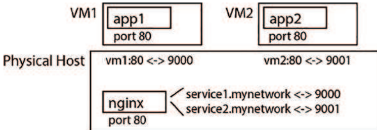
Figure 3.8. Microservice Architecture
